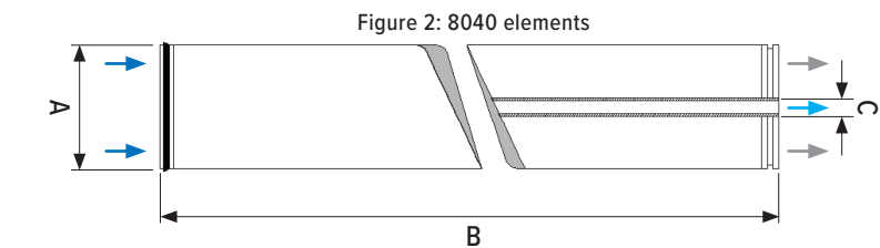
Figure 2: 8040 elements
